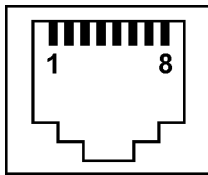
RJ45 socket (front view of the socket)
